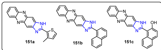
Scheme 39 Synthesis of 1-aryl-imidazo[4,5- b ] phenazine 151 .
