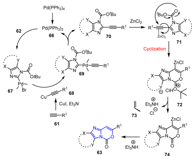
Scheme 16 Sonochemical coupling-cyclization mechanism for the synthesis of imidazo-1,3-oxazines 63 .
