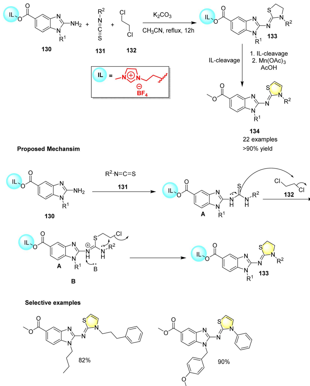
Scheme 32 Synthesis of thiazole using novel ionic liquid-tagged aminoethyl-functionalized imidazolium salt.
