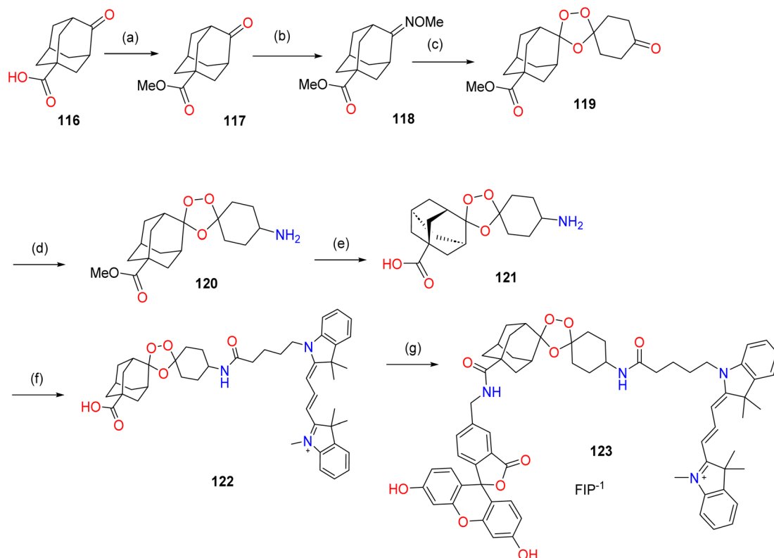
Fig. 23 Synthetic route of \text{FIP}^{-1} .
