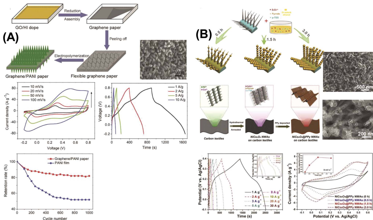
Fig. 11 Comparison between two papers including 3D spinel structured materials where one shows schematic illustrations of the fabrication process of hierarchical mesoporous \text{NiCo}_2\text{O}_4 @PPy hybrid NWAs on carbon textiles (B) and other shows 2D schematic illustrations of the formation process of graphene-PANI paper (A) and also comparing with the TEM and SEM images, CV curves at different compositions and times, Galvano-static charge discharge curves at different compositions and current densities, and cycle stability with capacitance retention value within multidimensional devices (Table 4). 78,92 [Reproduced from ref. 78 with permission from Elsevier, copyright 2025 and ref. 92 with permission from The Royal Society of Chemistry, copyright 2025].
