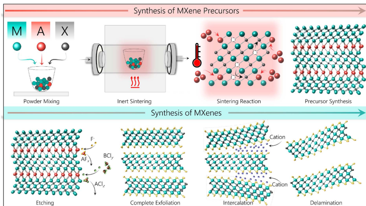
Fig. 3 The synthesis of different MXene precursors and MXenes (reproduced with permission from ref. 48 Copyright 2023, Elsevier).
