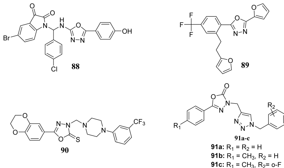
Fig. 17 Compounds (88–91).
