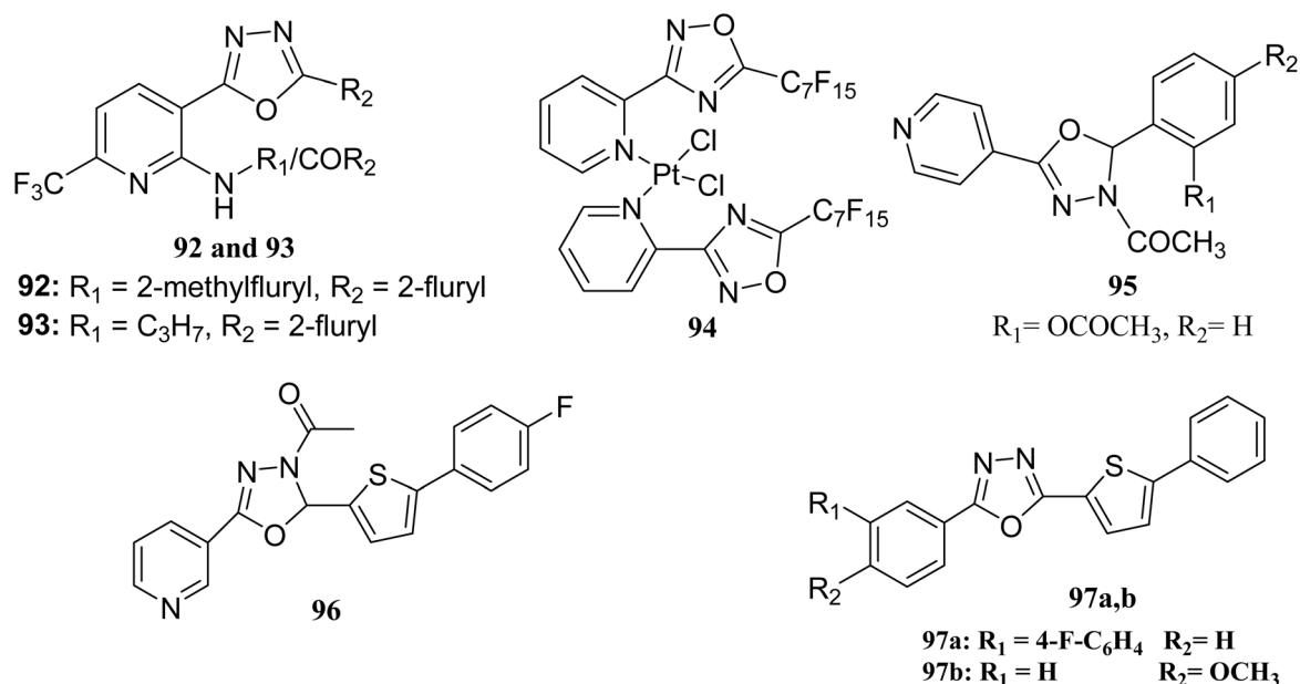
Fig. 18 Compounds (92–97).
