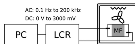
Fig. 2 Flow diagram of the experimental setup consisting of the LCR meter and magnetic fluid (MF) in the plate capacitor placed in a laboratory oven.
