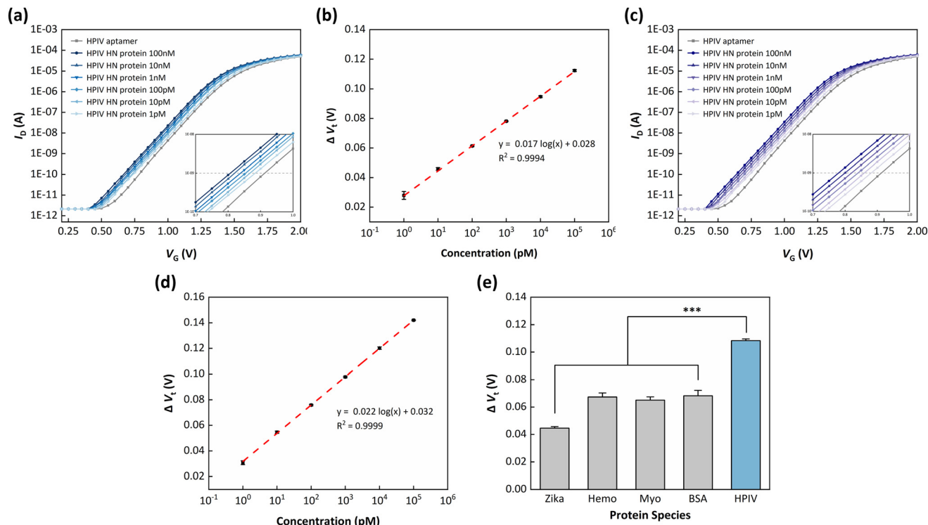
Fig. 5 (a) I_D-V_G curves by HPIV HN protein concentration (diluted in DIW). (b) Calibration curve of \Delta V_t values according to HPIV HN protein concentration (diluted in DIW). (c) I_D-V_G curves by HPIV HN protein concentration (diluted in 10% human serum). (d) Calibration curve of \Delta V_t values according to HPIV HN protein concentration (diluted in 10% human serum). (e) Selectivity test: comparison of significant differences between HPIV and non-target species ( p < 0.005 ).
