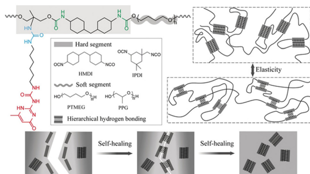
Fig. 7 Copolymers of hard and soft segments generate hierarchical H-bonding domains that are responsible for self-healing and energy dissipative properties. Figure adapted from ref. 44. Copyright 2018 Wiley-VCH Verlag GmbH & Co. KGaA, Weinheim.
