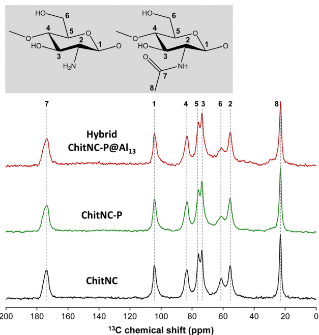
Fig. 11 13 C( 1 H) CP-MAS spectra of spray-dried microparticles obtained from different polysaccharide colloids: pristine chitin nanocrystals (ChitNC), phosphorylated ChitNC (ChitNC-P), and ChitNC-P in interaction with Al 13 (ChitNC-P@Al 13 ). The spectra were recorded at \nu_0(^{13}\text{C}) \equiv 75.4 MHz and \nu_{\text{MAS}} = 12 kHz (see Experimental), acquiring 4096 scans.
