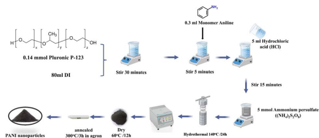
Fig. 10 Process for the hydrothermal synthesis of pure polyaniline (PANI).
