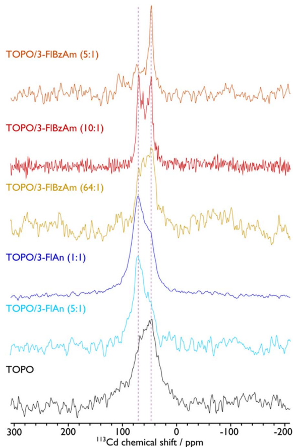
Fig. 4 ^{113}\text{Cd} MAS NMR spectra of CdS NCs with ligands indicated. A MAS frequency of 8 kHz was used for TOPO, 10 kHz was used for TOPO/3-FIAn (1 : 1), and 12 kHz was used for TOPO/3-FIAn (5 : 1), TOPO/3-FIBzAm (64 : 1), TOPO/3-FIBzAm (10 : 1), and TOPO/3-FIBzAm (5 : 1) CdS NCs. Vertical dashed lines highlight peak positions for wurtzite ( \sim 48 ppm) and sphalerite ( \sim 71 ppm) CdS NCs. See the ESI† for corresponding spectral fittings. Ratio of TOPO : fluorinated amine are by mass, as in Table 1.
