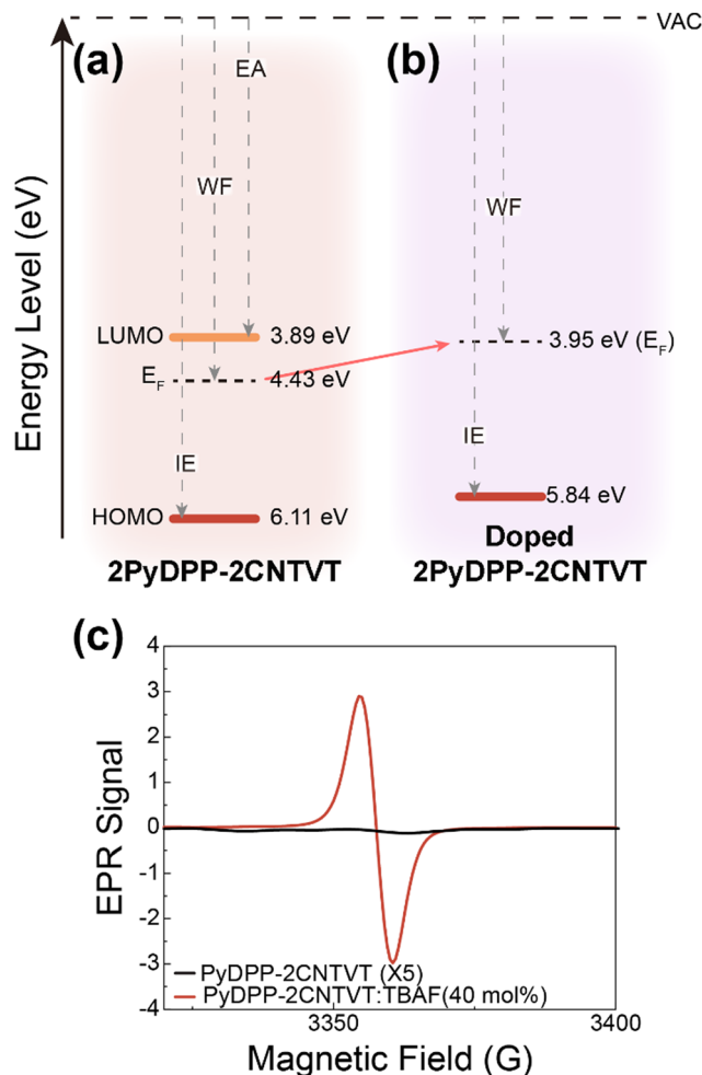
Fig. 4 Energy-level diagram of (a) pristine and (b) TBAF-doped (40 mol%) 2PyDPP-2CNTVT polymer films. (c) EPR spectra of pristine (black line, magnified 5 times) and doped (red line) polymer films.
