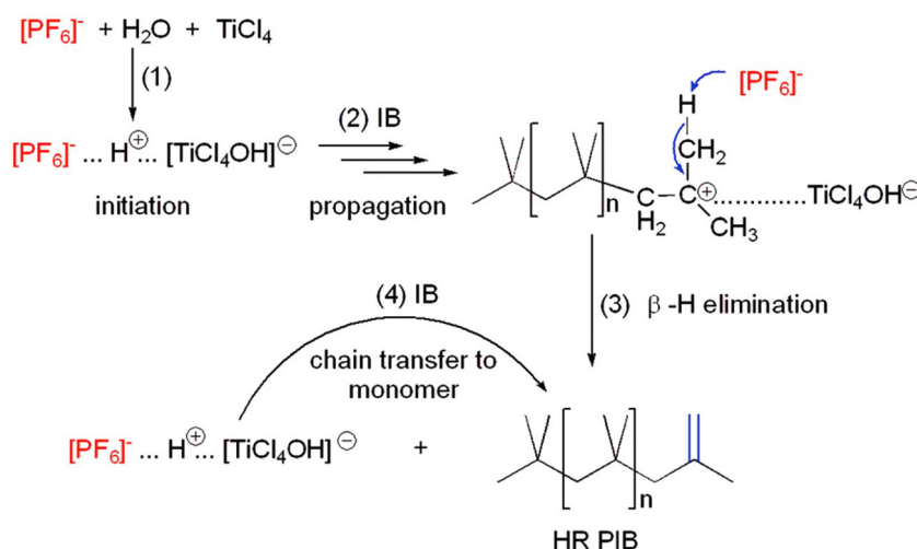
Fig. 2 Feasible mechanism of \text{H}_2\text{O}/\text{TiCl}_4 -initiated cationic polymerization of isobutylene in [Bmim][PF 6 ] ionic liquid at –10 °C. Reproduced from ref. 30 with permission from Royal Society of Chemistry, copyright 2019.
