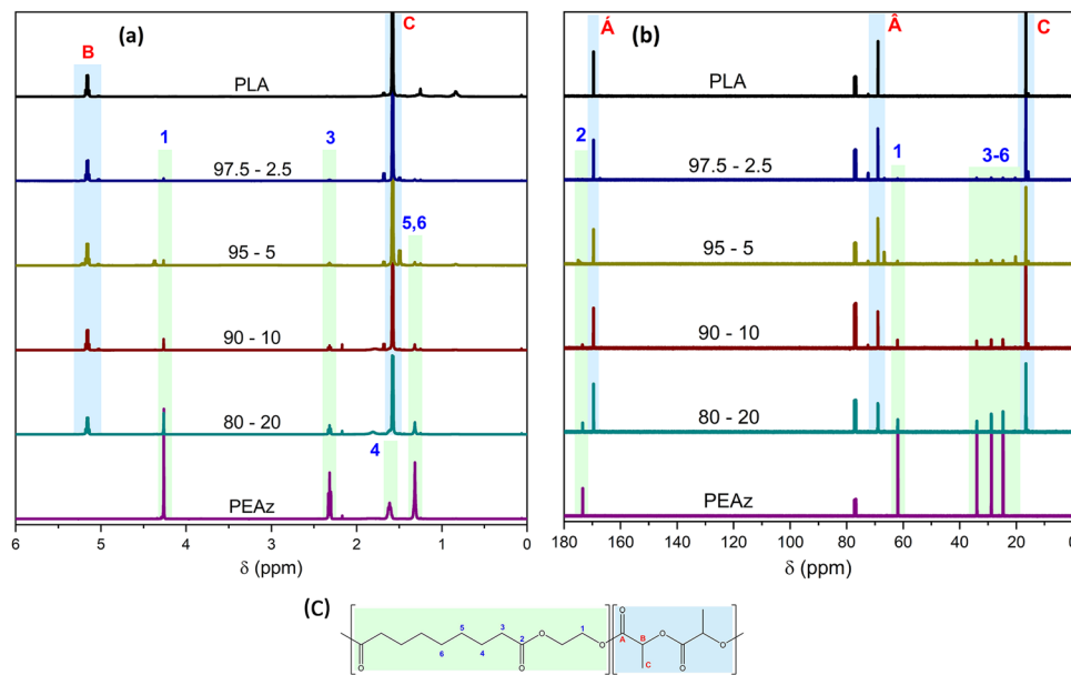
Fig. 3 (a) 1 H NMR, (b) 13 C NMR spectra of the synthesized homopolyesters and copolyesters, and (c) the corresponding signal assignments.
