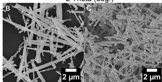
Fig. 12 (A) XRD patterns of the as-prepared YCMO and YNMO nanorods, and SEM images of (B) YNMO and (C) YCMO nanorods. 65 Copyright 2022, American Chemical Society.
