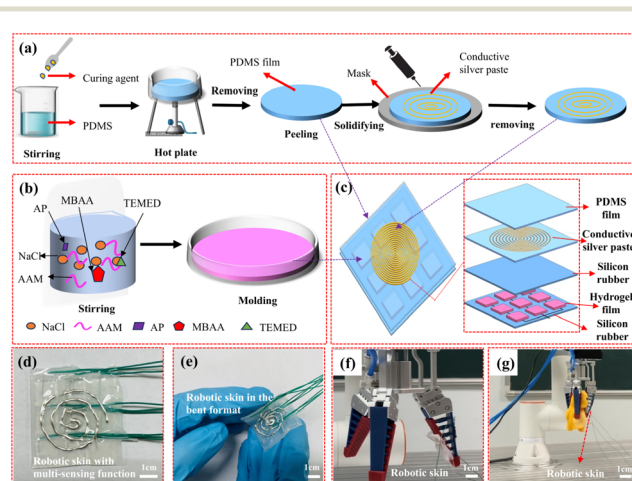
Fig. 2 (a) Material preparation of FDMSs with the proximity sensor. (b) Fabrication process of the AAM/NaCl hydrogel for the TENG pressure sensor. (c) Schematic diagram of the assembly process of FDMSs with a multi-layer structure. (d) Optical image of an FDMS with proximity distance and contact pressure-sensing function ability. (e) Optical image of an FDMS in the bent format. (f) Optical image of the robot finger with FDMSs. (g) Optical image of the robot finger in the grasping process.
