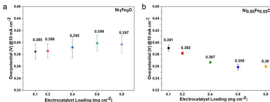
Fig. 7 Overpotentials of (a) \text{Ni}_1\text{Fe}_0\text{O} and (b) \text{Ni}_{0.95}\text{Fe}_{0.05}\text{O} measured at 10 mA \text{cm}^{-2} . The effect of different electrocatalyst loadings on the OER electrocatalytic activity is reported.
