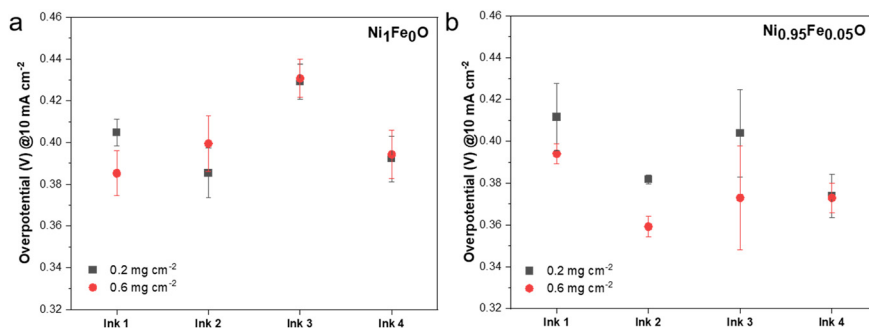
Fig. 6 OER overpotentials of (a) \text{Ni}_1\text{Fe}_0\text{O} and (b) \text{Ni}_{0.95}\text{Fe}_{0.05}\text{O} measured at 10 mA \text{cm}^{-2} . The effect of different ink formulations on the OER electrocatalytic activity is reported.
