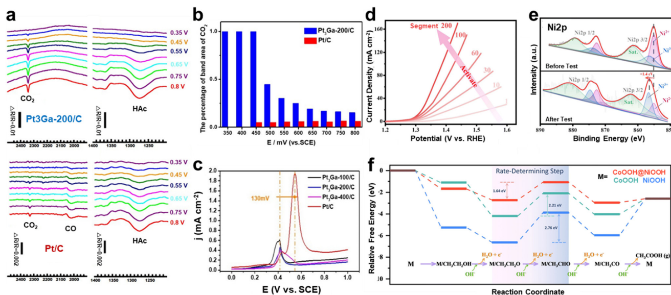
Fig. 4 Ethanol oxidation reaction (EOR). (a) In situ MSFTIR spectra of Pt 3 Ga-200/C and Pt/C for CO 2 and HAc during the EOR. (b) The percentage of band area of CO 2 (S CO 2 /S CO 2 + S HAc ). (c) CO-stripping voltammetry of catalysts in 0.1 M HClO 4 . (a–c) Adapted with permission. 59 Copyright 2023, American Chemical Society. (d) LSV activation curve of Co(OH) 2 @Ni(OH) 2 . (e) Ni 2p XPS spectra before and after electrochemical activation. (f) EOR free energy diagram for CoOOH, NiOOH and CoOOH@NiOOH based on DFT calculations. (d–f) Adapted with permission. 61 Copyright 2023, The Royal Society of Chemistry.
