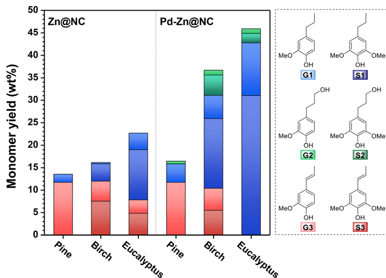
Fig. 11 Comparison of the yields of major monomers from different wood powders of the reaction over two catalysts: Zn@NC and Pd-Zn@NC. Reaction conditions: sawdust (50 mg), catalyst (6.5 mg), MeOH (10 mL), H 2 (3 MPa), 240 °C, and reaction time: pine, 4 h; birch, 8 h; eucalyptus, 12 h.
