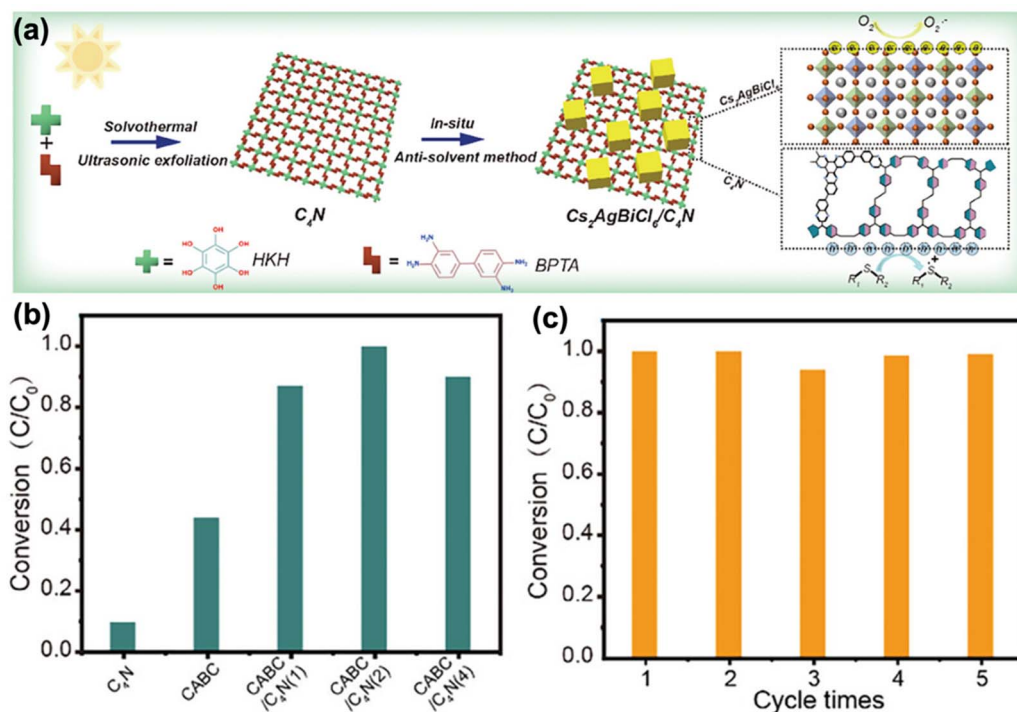
Fig. 18 (a) Schematic of synthesis path of the CAB/C 4 N heterojunction. (b) Comparison of photocatalytic oxidation properties of thioesters. (c) Photocatalytic cycle stability of CAB/C 4 N. Adapted with permission. 171 Copyright 2024, Wiley-VCH.
