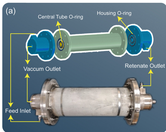
Fig. 16 Spiral wound module test rig for facilitated transport membrane assisted decarbonization; (a) schematic of the module's housing, (b) test setup (reproduced from ref. 197 with permission from Elsevier, copyright 2025).
