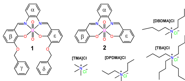
Scheme 1 The salophen- \text{UO}_2 complexes 1 and 2 and the tetraalkylammonium chloride salts [TMA]Cl, [DPDMA]Cl, [DBDMA]Cl and [TBA]Cl considered in the present work. The ring code is attributed assuming compounds 1 and 2 facing the reader with their convex side (see also Fig. 1a).
