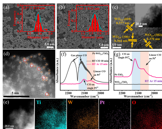
Fig. 1 SEM image and statistical analysis on particle size of (a) \text{TiO}_2 microspheres and (b) Pt- \text{WO}_{2.9}/\text{TiO}_2 ; (c) HRTEM image (inset: TEM image); (d) AC-HAADF-STEM image and (e) EDS elemental mapping of Pt- \text{WO}_{2.9}/\text{TiO}_2 ; CO-DRIFTS for (f) Pt- \text{WO}_{2.9}/\text{TiO}_2 and (g) Pt- \text{TiO}_2 , \text{WO}_{2.9}/\text{TiO}_2 .
