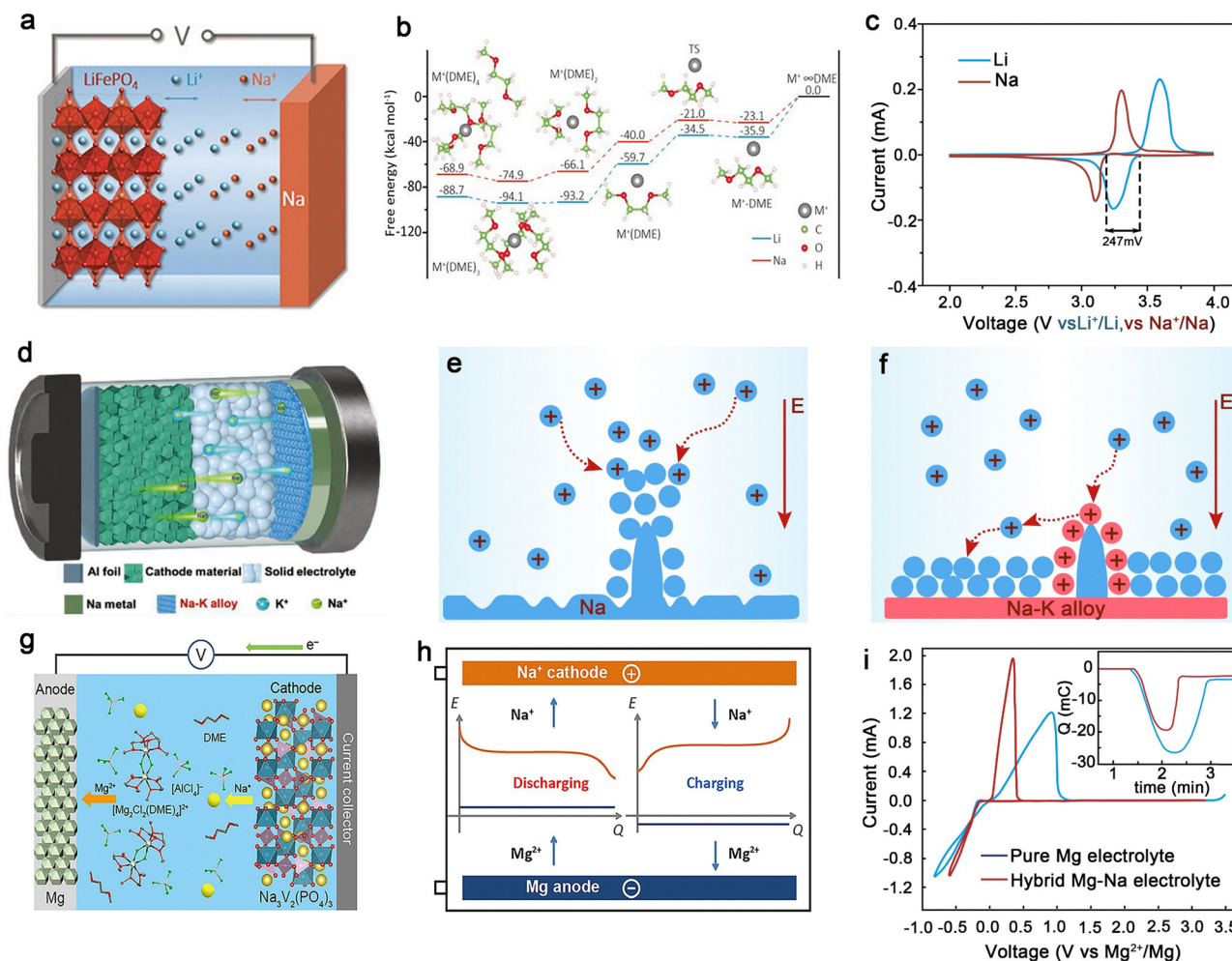
Fig. 4 (a) Schematic illustration of the Li–Na HIBs. (b) Free energy profiles and optimized geometries calculated for the solvation of Li + and Na + . (c) CVs of the Li metal batteries and the Li–Na hybrid batteries. Reproduced with permission from ref. 37. Copyright 2018, Wiley. (d) A strategy of locally targeting an anchor (LTA) with self-healing properties for all-solid-state sodium metal batteries. (e) Evolution process of interface during cycling process without LTA treatment. (f) Evolution process of interface during cycling steps via LTA treatment. Reproduced with permission from ref. 46. Copyright 2023, Wiley. (g) Electro-active species involved during charging a hybrid battery made of a Na 3 V 2 (PO 4 ) 3 cathode, a Mg anode, and an electrolyte of 0.2 M [Mg 2 Cl 2 ][AlCl 4 ] 2 and 0.4 M NaAlCl 4 in DME. (h) Illustration of the operating principle of a Mg–Na HIBs. (i) Cyclic voltammograms of a pure Mg electrolyte and a hybrid Mg–Na electrolyte in a three-electrode cell. Inset shows the accumulated charge during Mg deposition–dissolution cycle. Reproduced with permission from ref. 53. Copyright 2017, Elsevier.
