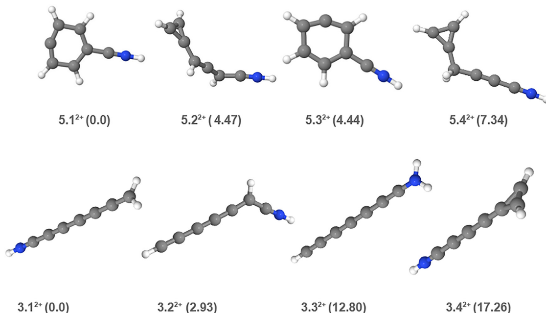
Fig. 5 Low-energy isomers of \text{C}_6\text{H}_5\text{CN}^{2+} ( m/z = 51.5 ) (top) and \text{C}_6\text{H}_3\text{CN}^{2+} ( m/z = 50.5 ) (bottom) obtained with the ABCluster software combined with DFT computations. Carbon atoms are gray, hydrogen atoms are white and nitrogen atoms are blue. The numbers in parentheses are the relative energies in \text{kcal mol}^{-1} obtained at the CCSD(T)/cc-pVTZ level of theory. Energy parameters and T1 diagnostics are shown in Tables S8 and S9 (SI).
