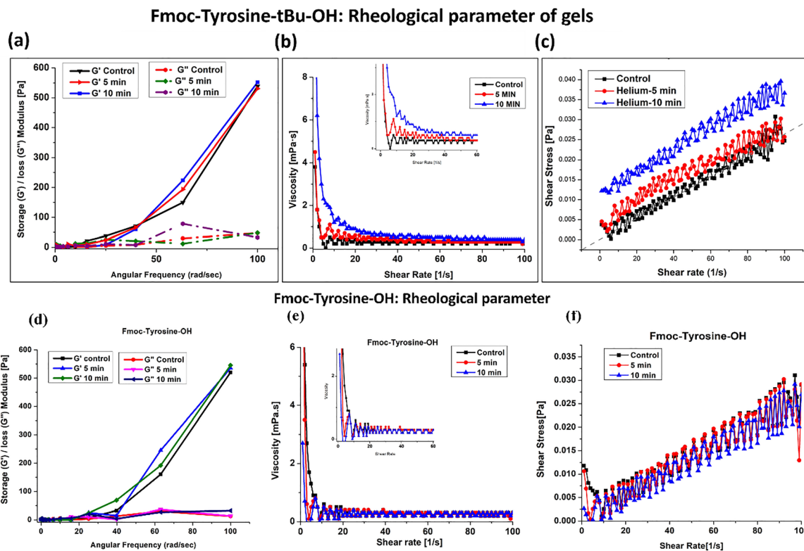
Fig. 3 Rheological analysis (a)–(c) of untreated and treated Fmoc-Tyr(tBu) samples and (d)–(f) Fmoc-Tyr-OH samples.
