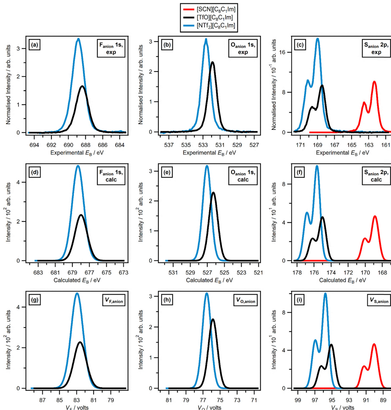
Fig. 4 Experimental and calculated data for [A][C 8 C 1 Im] where [A] − = [SCN] − , [TfO] − and [NTf 2 ] − . Experimental core-level XPS: (a) F 1s, (b) O 1s, (c) S 2p. Calculated core-level XPS: (d) F 1s, (e) O 1s, (f) S 2p. Electrostatic potential at nucleus: (g) V F , (h) V O , (i) V S . Experimental XP spectra are area normalised and charge referenced using methods given in SI, Section S4. Calculated XP spectra and V n data are charge referenced using methods given in SI, Section S4.
