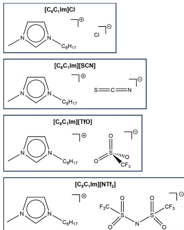
Fig. 1 Structures of the four ILs studied here. From top to bottom: 1-octyl-3-methylimidazolium chloride ( [\text{C}_8\text{C}_1\text{Im}]\text{Cl} ), 1-octyl-3-methylimidazolium thiocyanate ( [\text{C}_8\text{C}_1\text{Im}][\text{SCN}] ), 1-octyl-3-methylimidazolium trifluoromethanesulfonate ( [\text{C}_8\text{C}_1\text{Im}][\text{TfO}] ) and 1-octyl-3-methylimidazolium bis(trifluoromethanesulfonyl)imide ( [\text{C}_8\text{C}_1\text{Im}][\text{NTf}_2] ).
