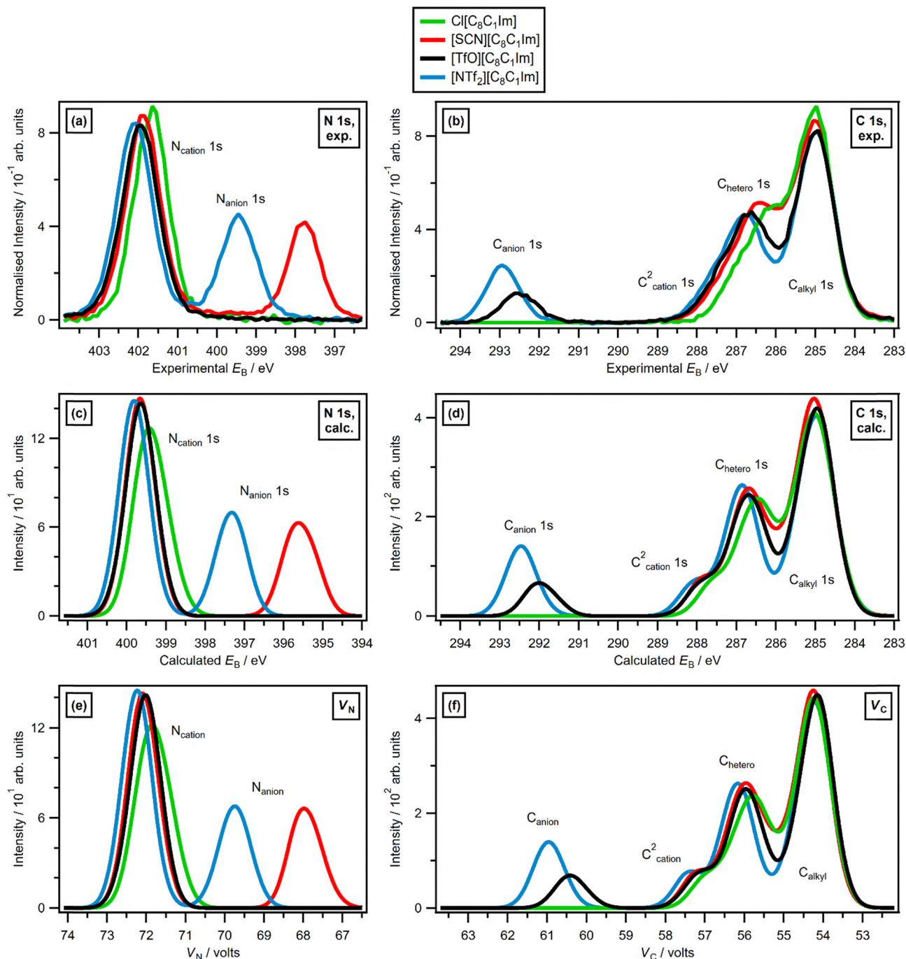
Fig. 3 Experimental and calculated data for [A][C_8C_1Im] where [A]^- = Cl^- , [SCN]^- , [TfO]^- and [NTf_2]^- . Experimental core-level XPS: (a) N 1s, (b) C 1s. Calculated core-level XPS: (c) N 1s, (d) C 1s. Electrostatic potential at nucleus: (e) V_N , (f) V_C . Experimental XP spectra are area normalised and charge referenced using methods given in SI, Section S4. Calculated XP spectra and V_N data are charge referenced using methods given in SI, Section S4.
