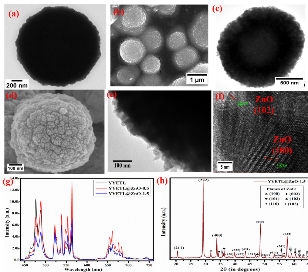
Fig. 4 FESEM, TEM, and HRTEM images of YYETL-ZnO-III- x microspheres for (a and b) 0.5 ml, (c)–(f) 1.5 ml of ZnO shell growth, (g) UCPL spectra of YYETL@ZnO-III- x microspheres and (h) XRD pattern of YYETL@ZnO-1.5 core-shell microspheres.
