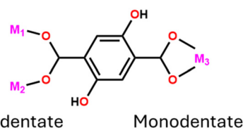
Fig. 4 Scheme of the bidentate and monodentate coordination modes of the DOBDC linker.
