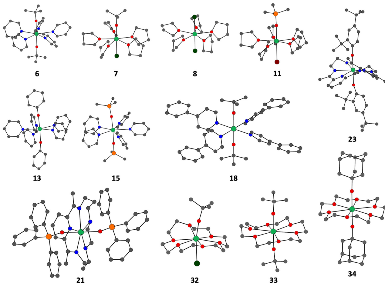
Fig. 4 Examples of bis-axial point charge complexes with the cations from [Dy(O t Bu) 2 (py) 5 ](BPh 4 ) ( 6 ), [Dy(O t Bu)Cl(THF) 5 ](BPh 4 ) ( 7 ), [DyCl 2 (THF) 5 ](BPh 4 ) ( 8 ), [Dy(OSiMe 3 )Br(THF) 5 ](BPh 4 ) ( 11 ), [Dy(OPh) 2 (py) 5 ](BPh 4 ) ( 13 ), [Dy(OSiMe 3 ) 2 (py) 5 ](BPh 4 ) ( 15 ), [Dy(O t Bu) 2 (4-Phpy) 4 ](BPh 4 ) ( 18 ), [Dy(OSiPh 3 ) 2 (N 5 -macro)](BPh 4 ) ( 21 ), [Dy(OPh t Bu) 2 (N 6 -macro)]PF 6 ( 23 ), [Dy(O t Bu)Cl(18-crown-6)](BPh 4 ) ( 32 ), [Dy(O t Bu) 2 (18-crown-6)] 3 ( 33 ) and [Dy(OAd) 2 (18-crown-6)] 3 ( 34 ). Dysprosium(III) = turquoise, bromine = brown, silicone = orange, chlorine = dark green, oxygen = red, nitrogen = blue, and carbon = grey; hydrogen atoms and counter ions have been omitted for clarity. 33–36,38–41,46,47
