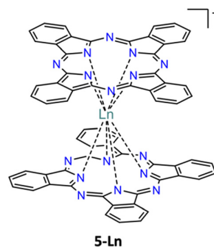
Fig. 3 Structure of the anion from ( n Bu 4 N)[Ln(Pc) 2 ] (5-Ln). 18
