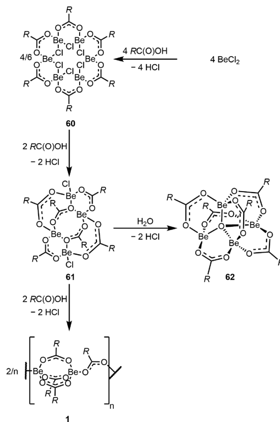
Scheme 12 Formation of beryllium chloro carboxylates and subsequent formation of homoleptic beryllium carboxylates as well as oxo-carboxylates (R = Ph, o-Tol, and Mes). 114
