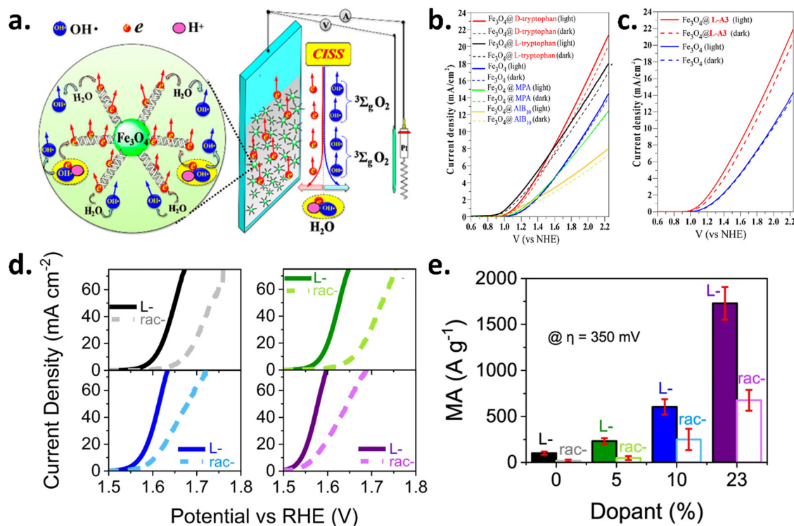
Fig. 6 Chiral functionalization of Fe 3 O 4 and Co 3 O 4 -based nanoparticles and enhancement of spin-selectivity for the OER. (a) Schematic of chiral-functionalized electrodes, where the C 1 S 2 effect enhances the OER via triplet oxygen production. (b) Photocurrent and dark current densities for Fe 3 O 4 NPs linked to chiral (D- and L-tryptophan) and achiral (mercaptopyronic acid, azo isobutyric acid) molecules, compared to pure Fe 3 O 4 NPs. (c) Photocurrent density of Fe 3 O 4 NPs linked to chiral L-A3 versus pure Fe 3 O 4 NPs. (d) LSV plot showing undoped (black) and iron-doped Rac- (dashed) and L-cobalt oxide (solid) nanoparticle catalysts in Nafion, with doping levels of 5% (green), 10% (blue), and 23% (purple), measured in 1 M NaOH. (e) Mass activity (MA) comparison of Rac- (open symbols) and L-cobalt oxide (filled symbols) nanoparticle catalysts in Nafion. Figures are adopted from ref. 24 and 26 with permission from American Chemical Society © 2018 and Nature © 2023.
