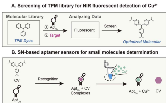
Scheme 1 (A) Schematic diagram of TPM dye screening for the NIR aptasensor and (B) the construction of the NIR aptasensor for \text{Cu}^{2+} detection.
