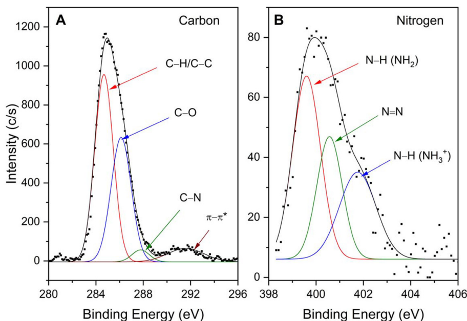
Fig. 3 High-resolution XPS spectra and deconvoluted peaks corresponding to (A) \text{C}_{1s} and (B) \text{N}_{1s} of the p -PDA-derived layer on the silica particles.
