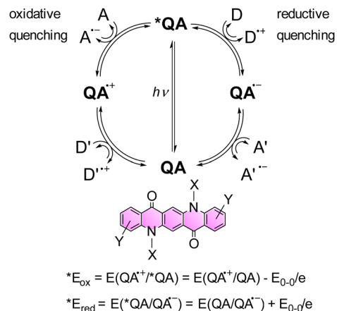
Scheme 3 Representation of possible reaction pathways of the *\text{QA} excited state through oxidative and reductive quenching, leading to the generation of oxidised \text{QA}^{*+} and reduced \text{QA}^{*-} , respectively. A and A' represent electron acceptors, while D and D' represent electron donors. The two equations enable the estimation of *E_{\text{ox}} and *E_{\text{red}} of the *\text{QA} excited state. 41,42
