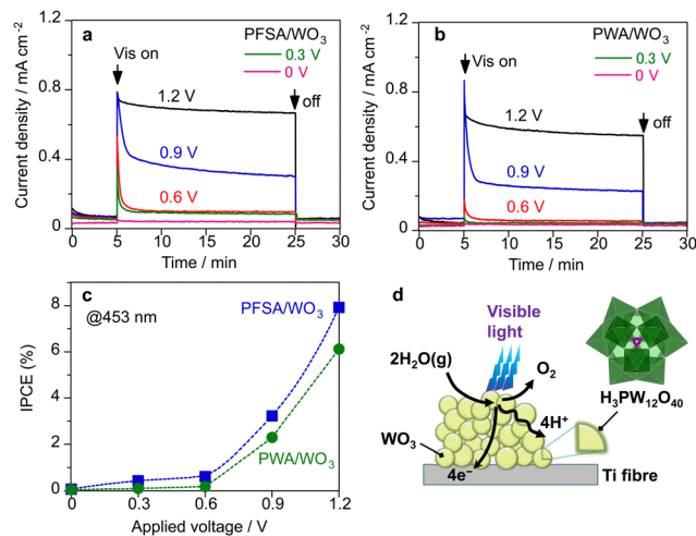
Fig. 5 Effect of applied voltage ( V vs. Pt–CB cathode) on the photocurrent response of (a) PFSA/ \text{WO}_3 and (b) PWA/ \text{WO}_3 in the vapour-fed PEM-PEC system under visible light ( 453\text{ nm} , 22\text{ mW cm}^{-2} ). (c) Steady-state IPCE at 453\text{ nm} after 20 min of photoirradiation. (d) Schematic illustration of PEC triple-phase boundary over the PWA/ \text{WO}_3 photoanode. The loading of PWA and PFSA were 5 and 12 wt% relative to \text{WO}_3 .
