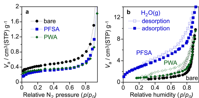
Fig. 6 (a) Nitrogen adsorption isotherms at -196\text{ }^\circ\text{C} and (b) water vapour adsorption-desorption isotherms at 25\text{ }^\circ\text{C} for bare \text{WO}_3 , PWA/ \text{WO}_3 , and PFSA/ \text{WO}_3 layers on Ti felt. The loading of PWA and PFSA were 5 and 12 wt% relative to \text{WO}_3 .
