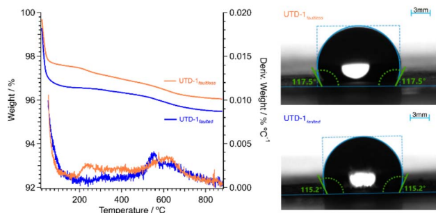
Fig. 2 (Left) Thermal gravimetric profiles for detemplated UTD-1 variants. Data gathered under air atmosphere. (Right) Water contact angle measurements for UTD-1 variants.
