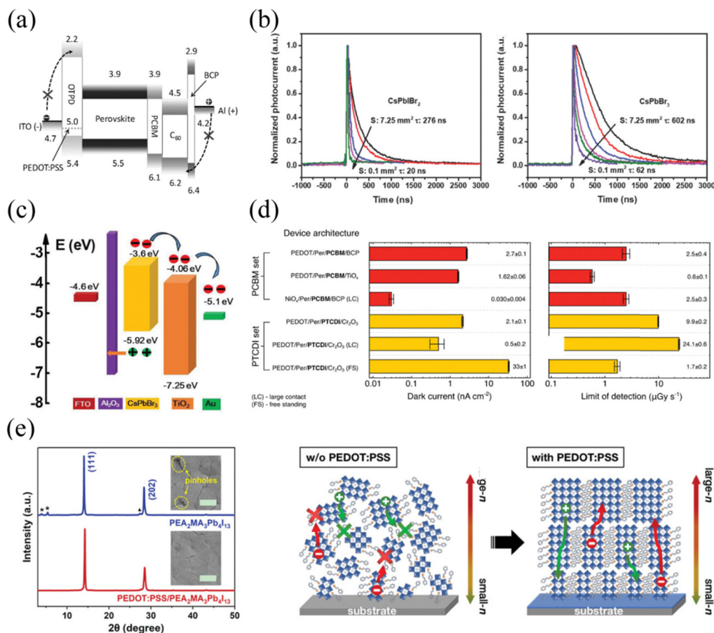
Fig. 10 (a) Energy diagram of the cross-linked OTPD MHPPDs. Reproduced with permission. 10 Copyright 2015, Wiley-VCH. (b) Transient response curves of the inorganic MHPPDs with PTA/PEIE. Reproduced with permission. 106 Copyright 2018, Wiley-VCH. (c) Energy band diagram of the MHPPDs with ultrathin \text{Al}_2\text{O}_3 and \text{TiO}_2 modification layers. Reproduced with permission. 107 Copyright 2019, Wiley-VCH. (d) Summary of the interface engineering based on several organic materials. Reproduced with permission. 108 Copyright 2020, Wiley-VCH. (e) XRD patterns of quasi-2D thin films without and with PEDOT:PSS interlayer (left), the insets are the corresponding top-view FESEM images (scale bar: 1 \mu\text{m} ), and schematic illustration of the orientational growth of MHP films without/with PEDOT:PSS interlayer. Reproduced with permission. 109 Copyright 2023, Wiley-VCH.
