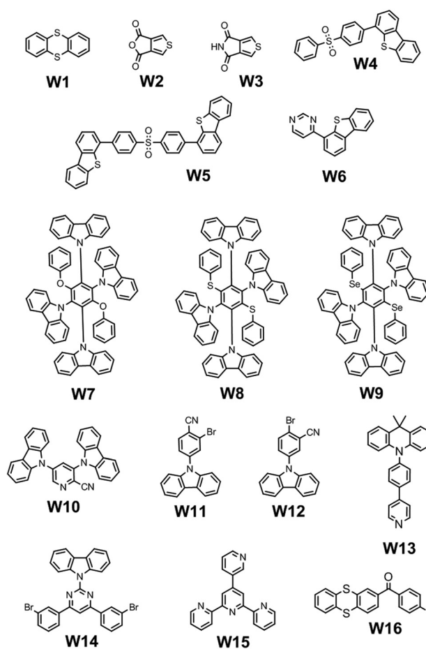
Fig. 20 Molecular structures of white RTP-agents W1–W16 .
