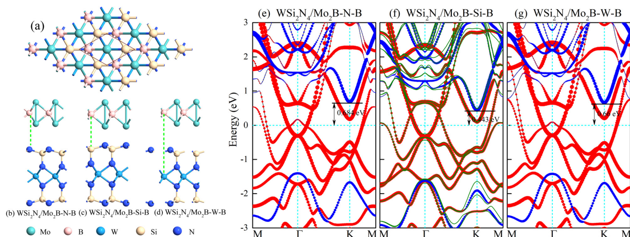
Fig. 1 (a) and (b)–(d) Top view and side view of the structures of WSi 2 N 4 /Mo 2 B heterostructures. (e)–(g) Projected band structures of WSi 2 N 4 /Mo 2 B heterostructures in three different stacking models. The red and blue lines denote the contributions from Mo 2 B and WSi 2 N 4 , respectively. The green lines represent the band structures with SOC.
