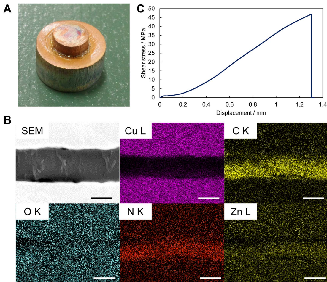
Fig. 4 Adhesive characterization of the ZIF-zni gel. (A) Photograph of the adhesive body. (B) Cross-sectional SEM image and EDX analysis of the adhesive body. Scale bar: 1 μm. (C) Stress-displacement curve of the adhesive body.
