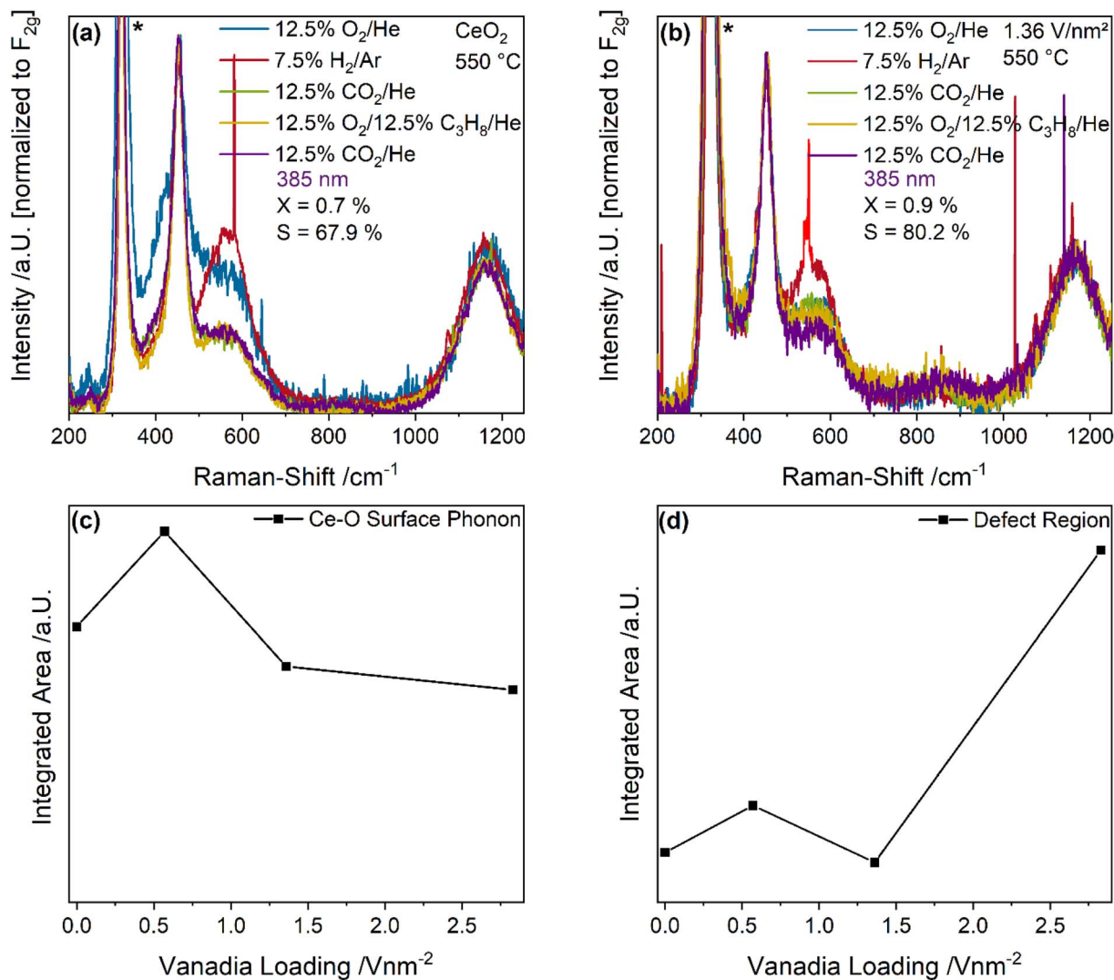
Fig. 4 UV-Raman spectra (385 nm excitation) of (a) \text{CeO}_2 and (b) the 1.36 \text{ V nm}^{-2} sample recorded under the indicated gas feeds at 550 °C. Spectra were normalized to the F_{2g} peak and the \text{CaF}_2 window signal is marked with an asterisk. Quantification of the (c) Ce–O surface phonon and (d) defect region changes between spectra recorded under 12.5% \text{CO}_2/\text{He} and 12.5% \text{CO}_2/12.5\% \text{C}_3\text{H}_8/\text{He} .
