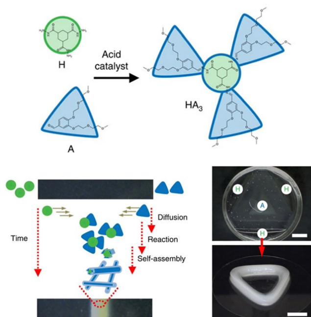
Fig. 37 Two-component gel formed by dynamic reaction between acyl-hydrazide (H) and aldehyde (A). Allowing diffusion to bring the two-components together within a pre-formed polymer gel matrix causes the LMWG to assemble with spatial resolution dependent on the starting locations of the H and A components. Figure adapted and reproduced from ref. 286a with permission of Springer Nature, © 2017.
