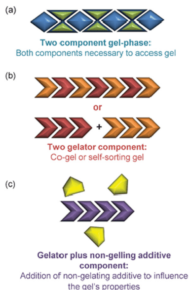
Fig. 18 Schematic of multi-component gels according to Buerkle and Rowan: (a) Two component gel phase, (b) Two gelator components, (c) Gelator plus non-gelling additive component, figure reproduced from ref. 173 with permission of the Royal Society of Chemistry, © 2012.
