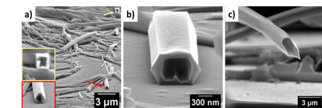
Fig. 5 FESEM images of 1 taken at an angle of 10^\circ from the surface showing the open end of the microtubular assembly. The images reveal that tubular assembly is (a) triangular, square, and (b) hexagonal in shape. Zoomed images are shown in the insets (red arrows showing triangular tubes and yellow arrows showing square-shaped tubes); (c) FESEM images of 5 taken at an angle of 10^\circ from the surface showing the open end of the microtubular assembly.
