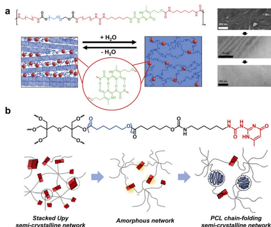
Fig. 3 (a) Hydration triggered crystal-phase evolution of multiblock PEG-based amphiphilic copolymers containing UPy moieties. Copyright 2014, American Chemical Society. Reproduced with permission from ref. 36. (b) Dual dynamic networks composed of quadruple H-bonds and crystalline physical interactions, whose morphology is determined using the arm-length. Copyright 2020, Elsevier. Reproduced with permission from ref. 40.
