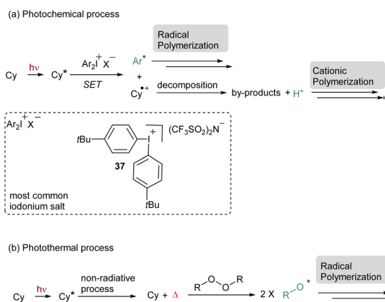
Scheme 10 General mechanism of NIR-polymerization with cyanines.
