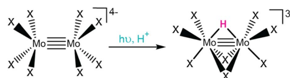
Fig. 6 Excited state protonation of [Mo 2 X 8 ] 4- yields [Mo 2 ( \mu -H)( \mu -X) 2 (X) 6 ] 3- .
