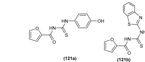
Fig. 51 1-(2-Furoyl)thiourea derivatives.
