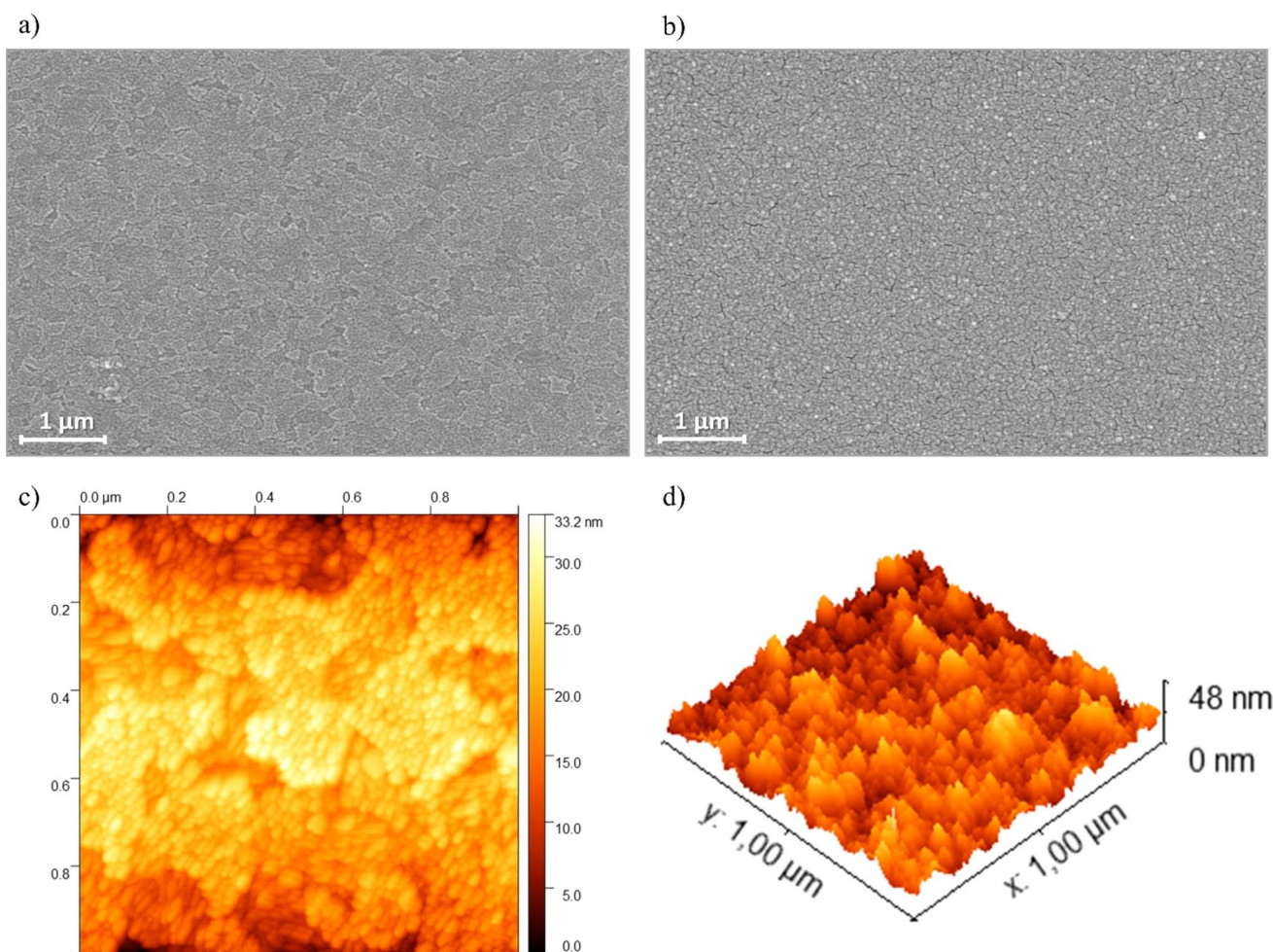
Fig. 6 SEM images of (a) bare ITO and (b) PEDOT-TPPF 16 film. Scale bars are 1 \mu\text{m} . (c) AFM images of ITO electrode surface (scan size 1 × 1 \mu\text{m} ) registered after electrodeposition of porphyrin film. (d) Three-dimensional representation of the electrode surfaces measured by AFM. Films were grown cycling in the same conditions of the exhibited in Fig. 3.
